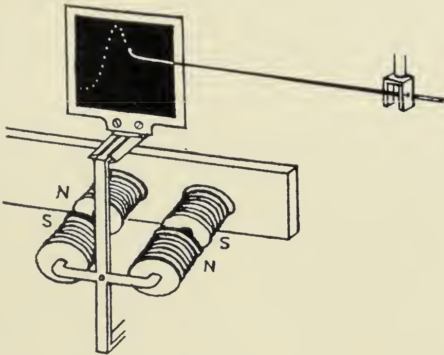
FIG. 11. Diagrammatic representation of the Electro-Oscillating Recorder. Electro-magnetic oscillating arrangement alone shown in the figure.
